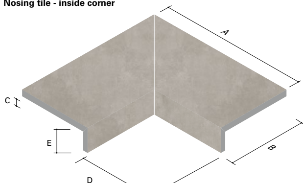
Schenkelplatte-Innenecke Nosing tile - inside corner
